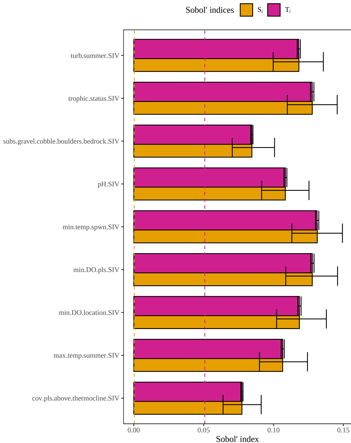
Figure 4. Results of a sensitivity analysis for the spottedbassLac model based on an arithmetic mean structure. Dashed lines represent baseline numerical approximation error for S_i and T_i ( i.e. , dummy variables).
